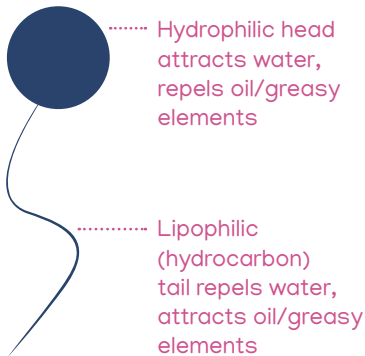
Surfactant molecule
