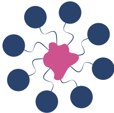
Micelles in the presence of dirt or grease
