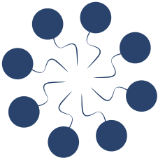
Surfactant molecules in water (solution)
