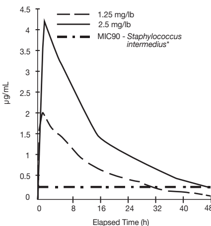
Figure 3: Mean plasma concentrations (µg/mL) following single oral administration of marbofloxacin to adult cats at a dosage of 2.5 mg/lb.
