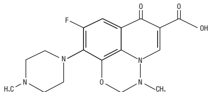
Figure 1: Chemical structure of marbofloxacin
